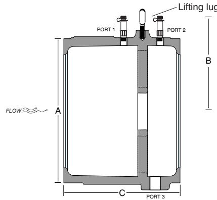
Model WS shown with standard lifting lug and standard Extended Pressure / Temperature Ports
