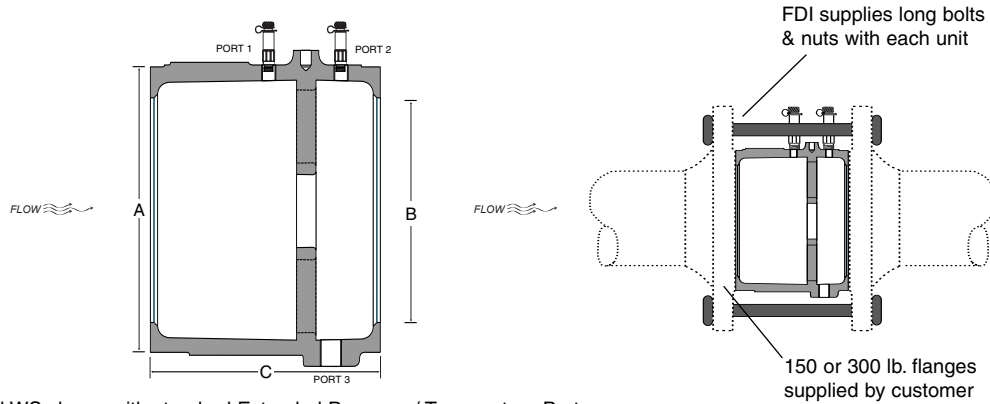
Model WS shown with standard Extended Pressure / Temperature Ports
