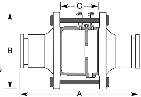
WG shown with standard SuperSeal P/T ports
