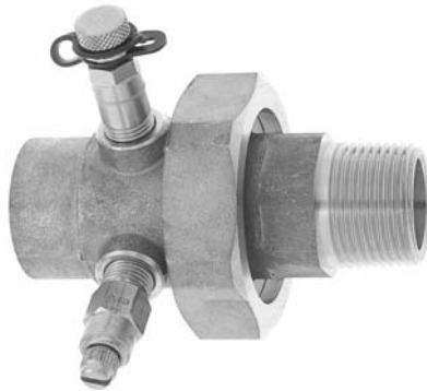
Model UP shown with optional Manual air vent and Pressure / Temperature port.
